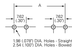
Straight Leads for 102 and 122 Series
