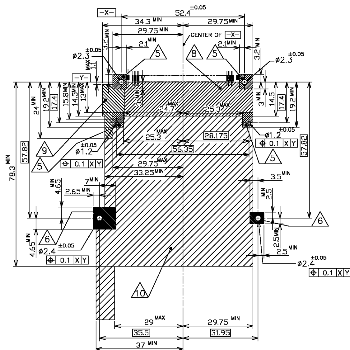
PCB LAYOUT VIEW C SCALE:1:1 CONNECTOR MOUNTING LAYOUT
