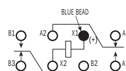
TERMINAL VIEW
