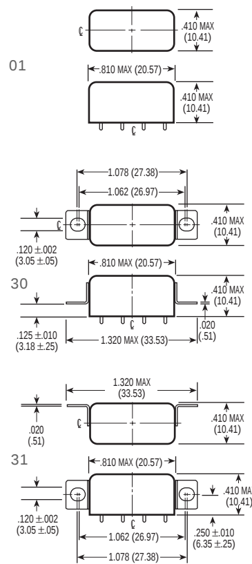
MOUNTING STYLES
