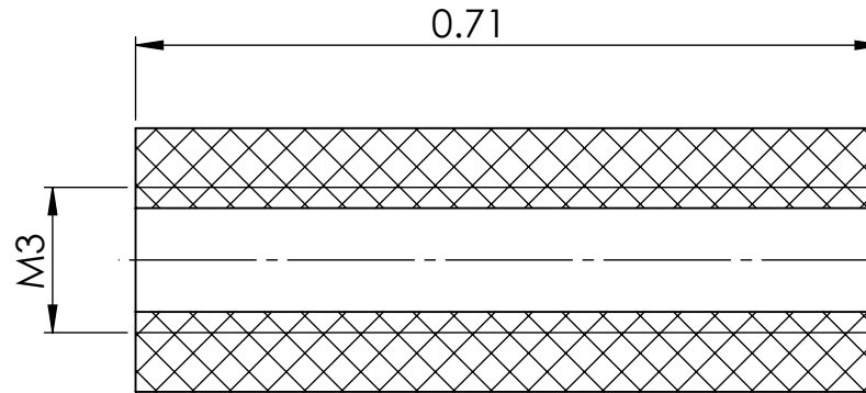
SECTION Y-Y
