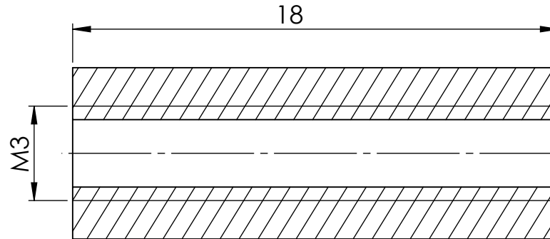
SECTION Y-Y
