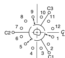
THREE POLE Styles M, MS, H and HS
