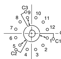
THREE POLE Styles A, D and S
