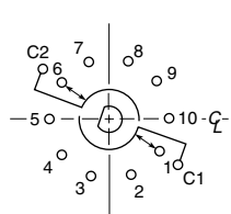
TWO POLE
