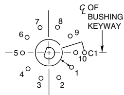
ONE POLE
