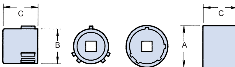
RECEPTACLE HOLDER
