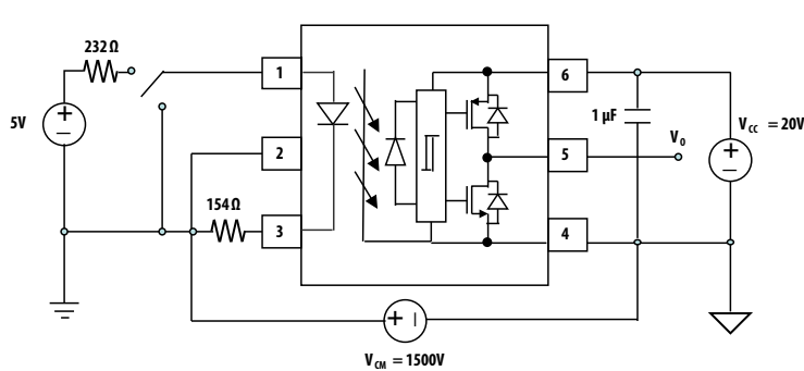
Figure 15: .CMR Test Circuit with Split Resistors Network
