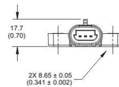
CONNECTOR - ELECTRICAL PINOUT
