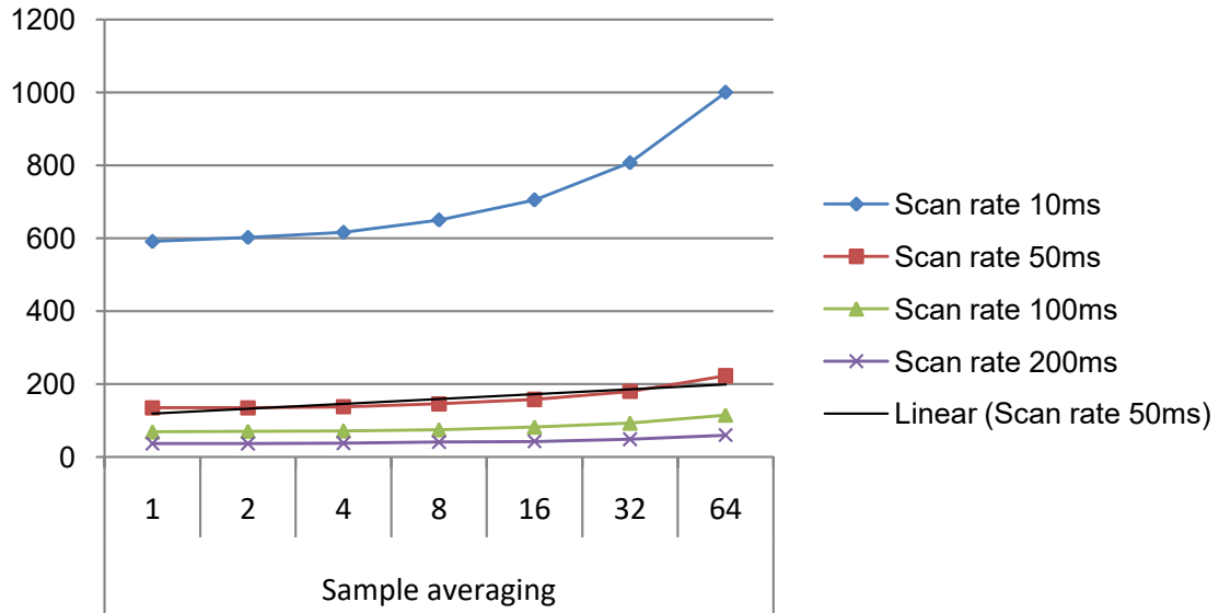
Figure 37-10. Power Consumption [ \mu A] 10 sensors, noise countermeasures Enabled, f=48\text{MHz} , V_{CC}=3.3\text{V}
