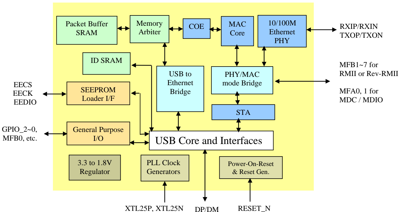
Figure 6 : Block Diagram
