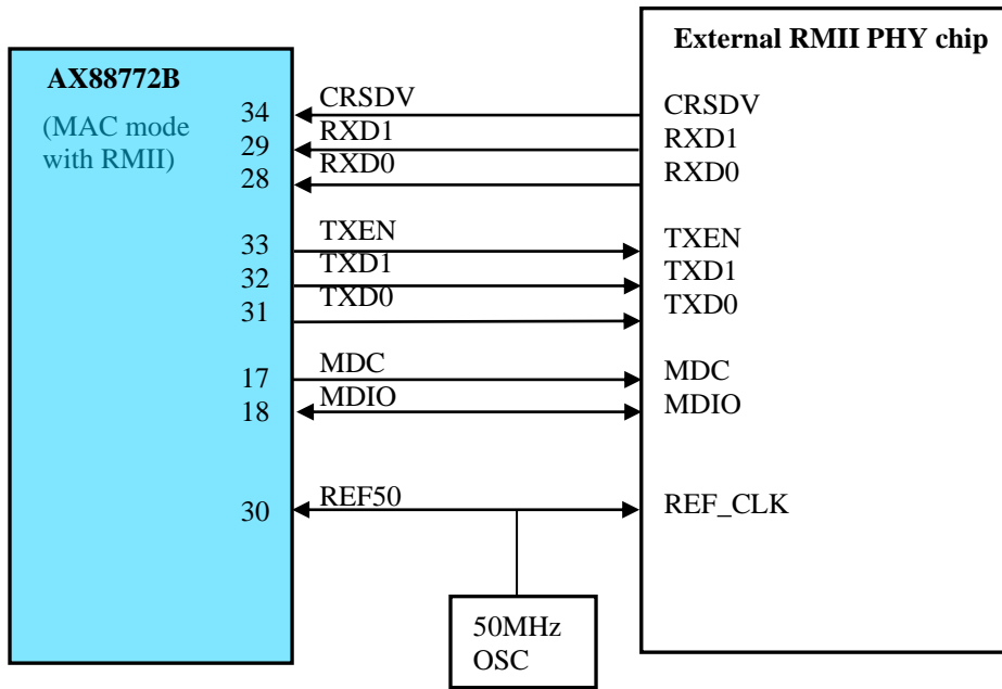
Figure 9 : RMIi to External PHY chip with 50MHz OSC
