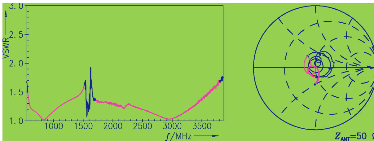
Figure 8: Reflection coefficient at ANT port.
