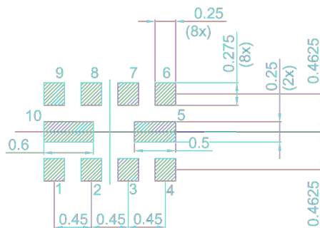
Figure 2: Drawing of package with package height A = 0.6 \text{ mm} (max.). See Sec. Package information (p. 24).
