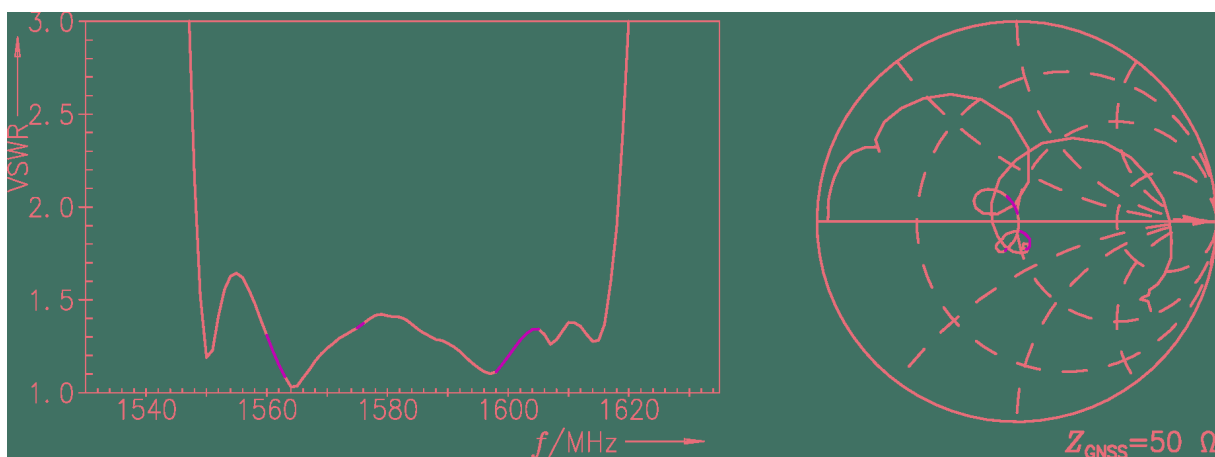
Figure 6: Reflection coefficient at GNSS port.
