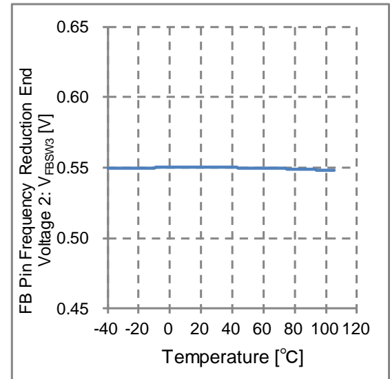
Figure 34. FB Pin Frequency Reduction End Voltage 2 vs Temperature
