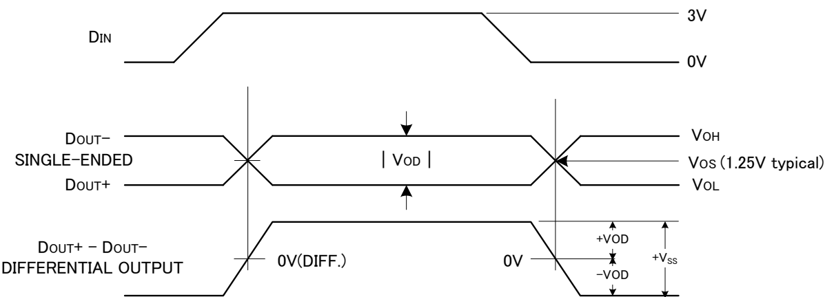
Figure 14. Driver Output Levels
