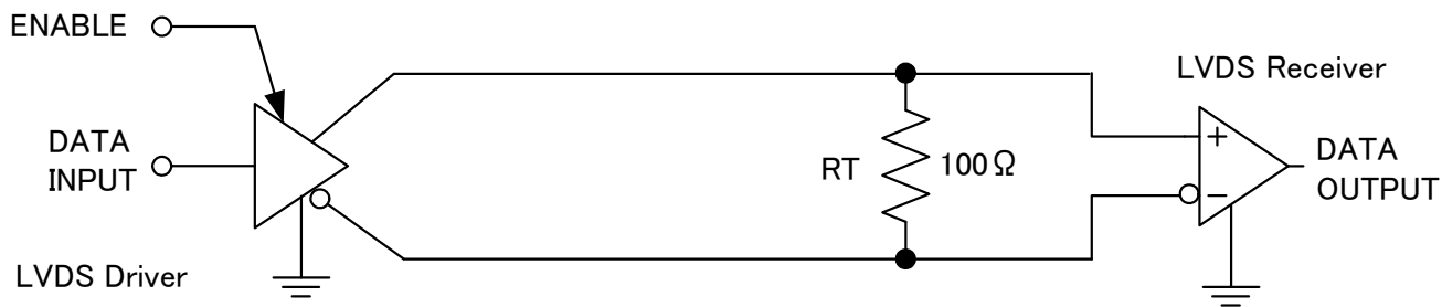
Figure 13. Point-to-Point Application
