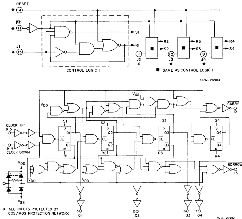
Fig. 2 - CD40193B logic diagram (binary).
