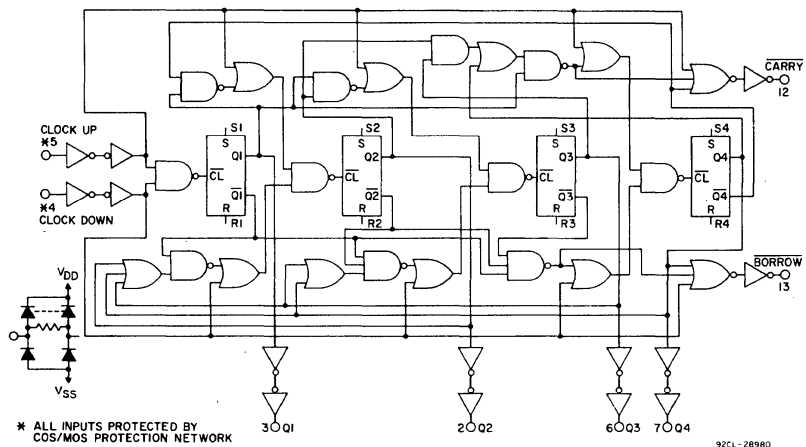
Fig. 1 — CD40192B logic diagram, (BCD).
