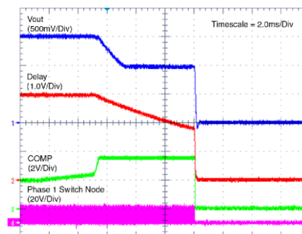
Figure 9. Over-Current Latch-Off Waveforms
