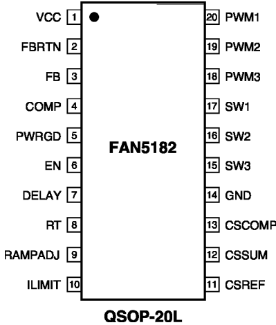
Figure 2. Pin Assignments
