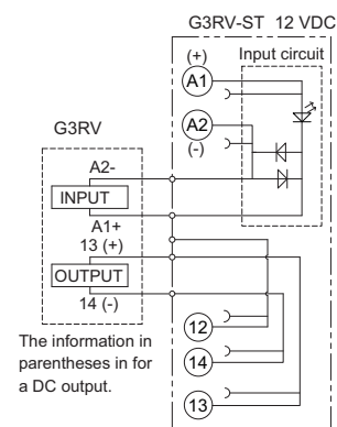
Terminal Arrangement/ Internal Connection Diagram (TOP VIEW)
