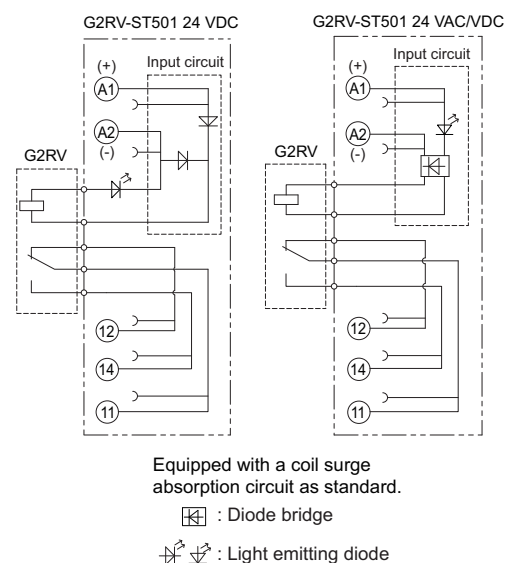
Terminal Arrangement/Internal Connection Diagram (TOP VIEW)
