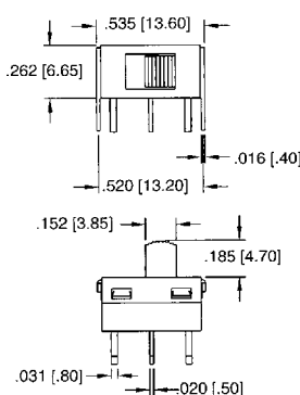
MECHANICAL OUTLINE
