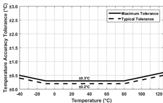
Figure 5. HS4011 Temperature Sensor Accuracy Tolerance
