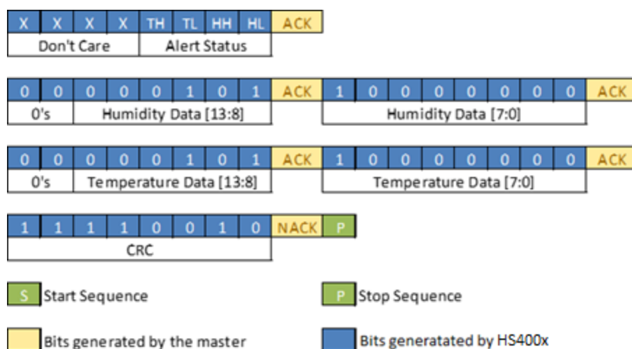
Figure 15. Data Returned from HS401x when the Alert Feature is Enabled in Periodic Measurement Mode
