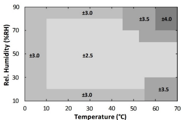
Figure 4. HS4013 RH Accuracy over Temperature
