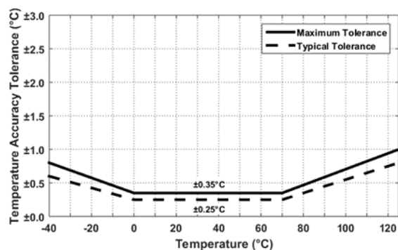
Figure 6. HS4013 Temperature Sensor Accuracy Tolerance
