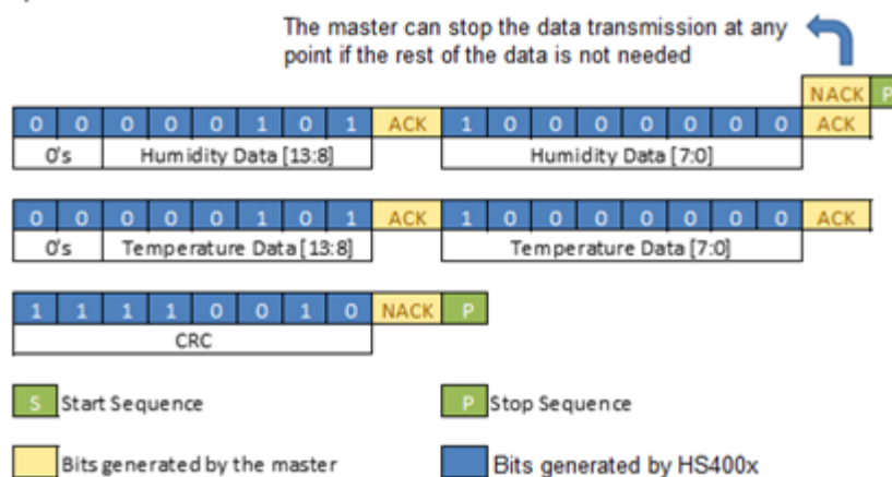
Figure 9. Typical Hold Measurement Sequence for a Humidity and Temperature Command
