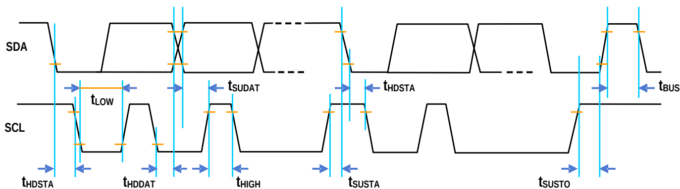
Figure 7. Timing Diagram
