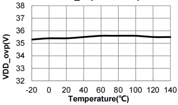
VDD_ovp vs. Temperature
