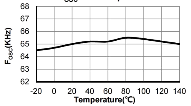
F OSC vs. Temperature
