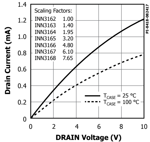
Figure 22. Output Characteristics.
