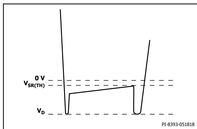
Figure 13. Acceptable FORWARD Pin Waveform After Handshake with SR Switch Conduction During Flyback Cycle.
