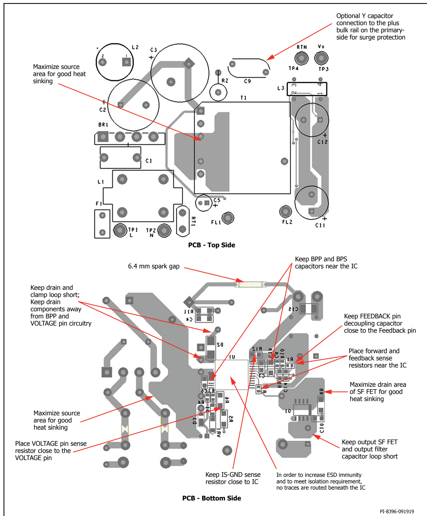
Figure 18. PCB.
