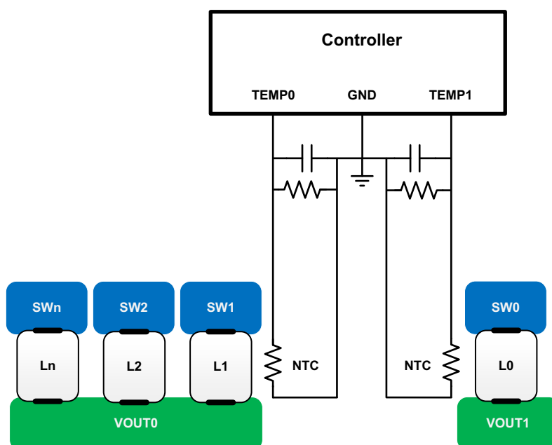
Figure 16. NTC Placement
