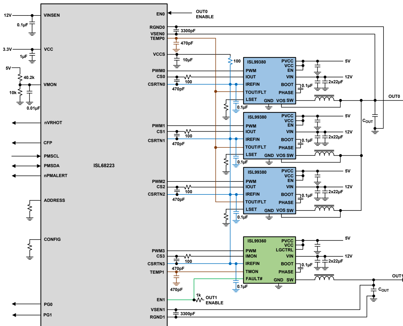
Figure 1. 3+1 Solution Using Smart Power Stage
