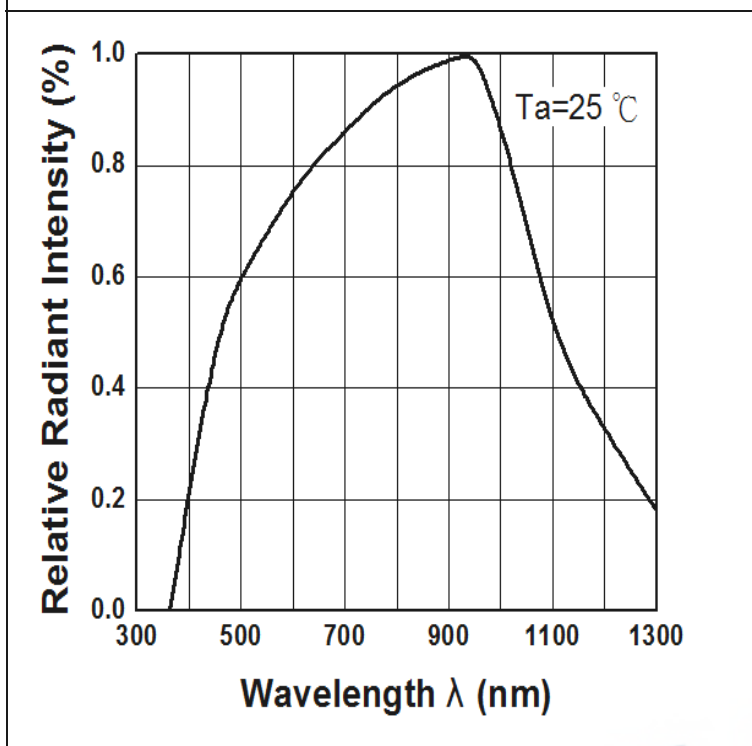
Spectral Sensitivity
