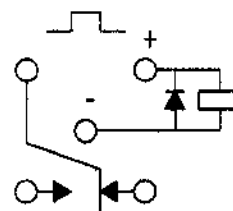
TERMINAL VIEW
