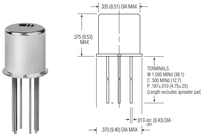
1MS/1MSD/1MSDD Enclosure
