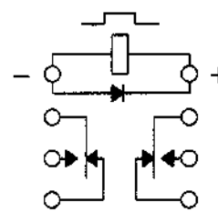
TERMINAL VIEW
