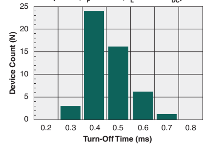
Typical Turn-Off Time (N=50, I_F=10\text{mA} , I_L=120\text{mA}_{DC} )
