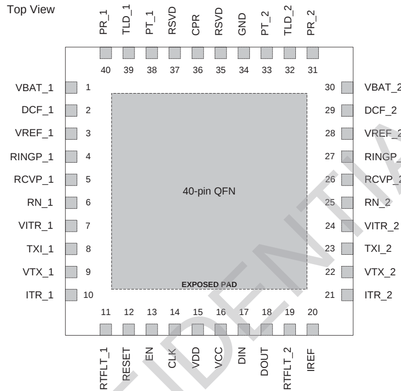
Figure 2 - 40 Pin QFN
