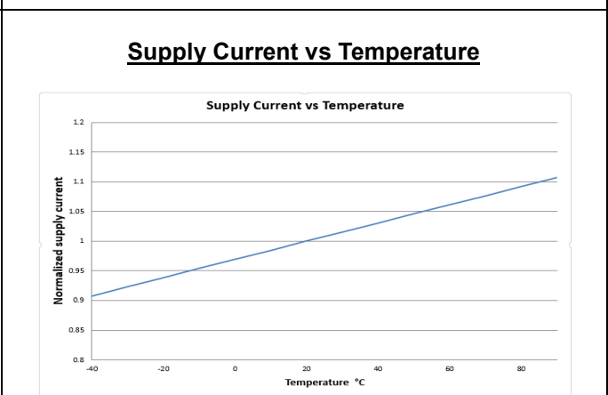
Figure 4.4 Supply Current vs Temperature
