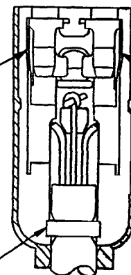
SECTION B-B
