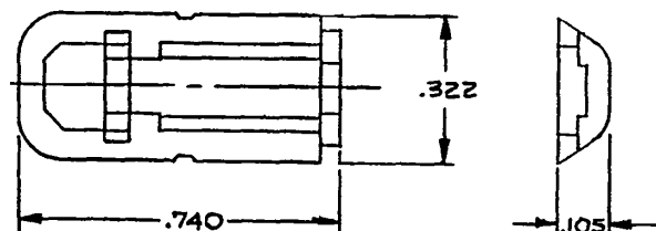
INSERT #3 MJ-103-3
