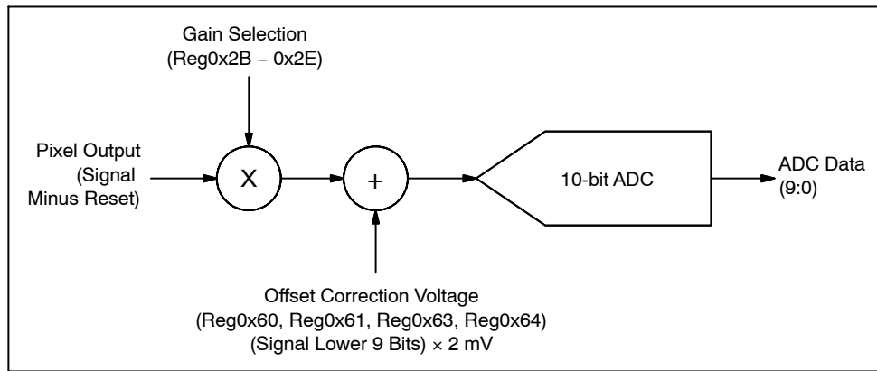
Figure 10. Signal Path
