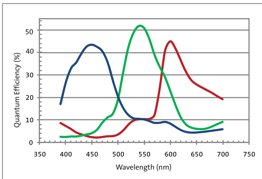
Figure 27: Quantum Efficiency
