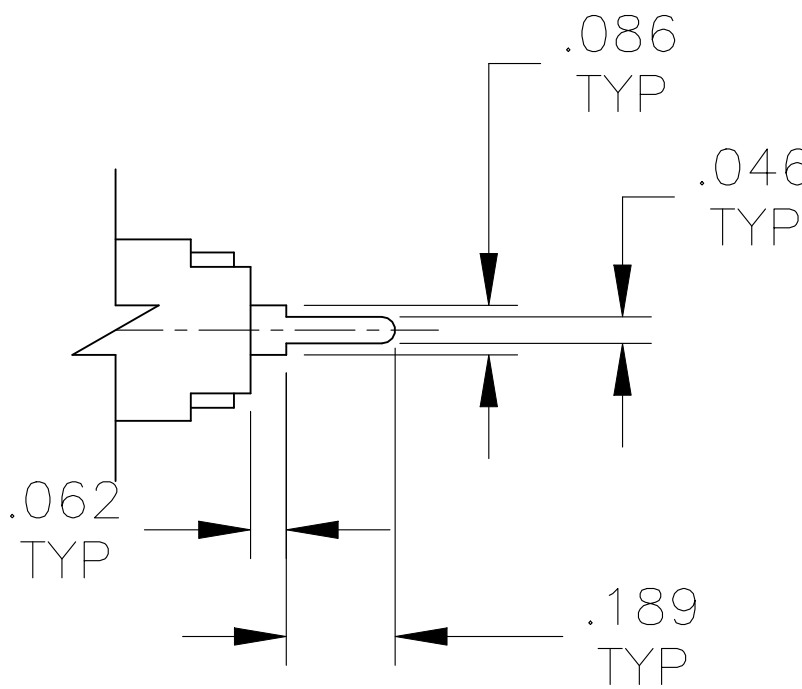
PC TERMINAL
