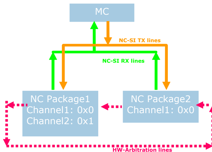
Figure 10-10 Multi-NC Environment
