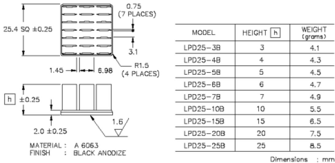
Figure 13-5 7mm Height Passive Heat Sink (Alpha Novatech, Inc. PN: LPD25-7B)
