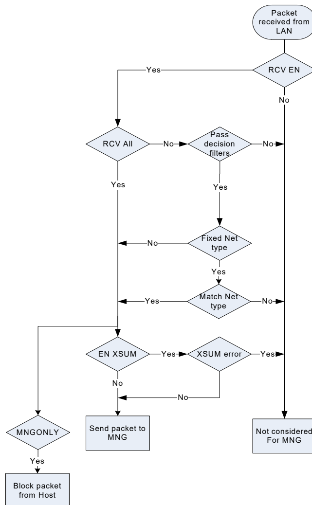
Figure 7-5 Manageability Filtering
