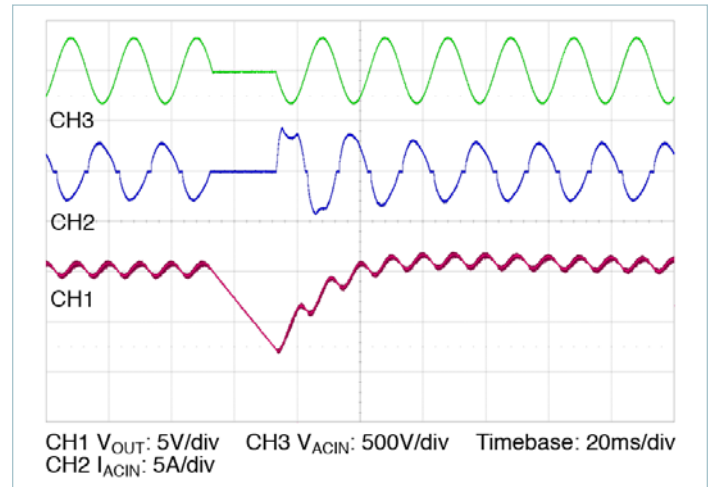
Figure 10 — Line drop out, 230V 50Hz, 0^{\circ} phase, I_{OUT} = 16.7A , C_{OUT} = 44,000\mu F
