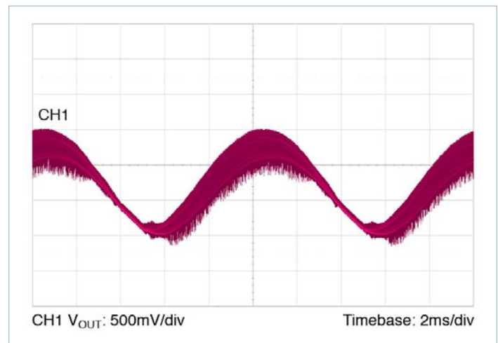
Figure 6 — Typical line frequency output voltage ripple waveform, T_{CASE} = 30^{\circ}\text{C} , V_{IN} = 230\text{V} , I_{OUT} = 16.7\text{A} , C_{OUT} = 44,000\mu\text{F} , 20MHz BW
