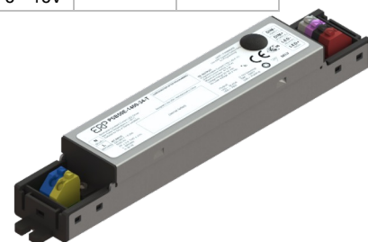
Terminal Blocks: "-T" Suffix L 154.2 x W 26.2 x H 21.85 mm (L 6.07 x W 1.03 x H 0.86 in.)
