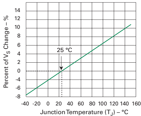
Normalized VS Change vs. Junction Temperature
