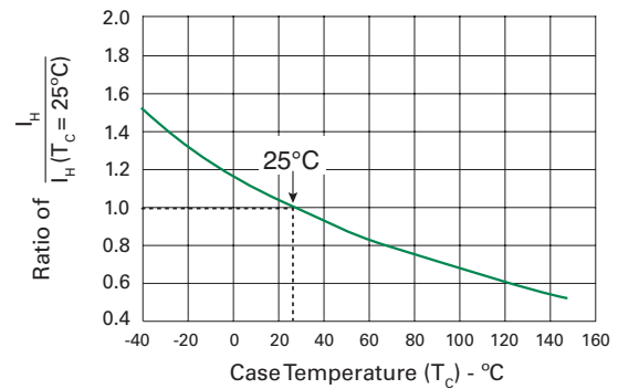
Normalized DC Holding Current vs. Case Temperature
