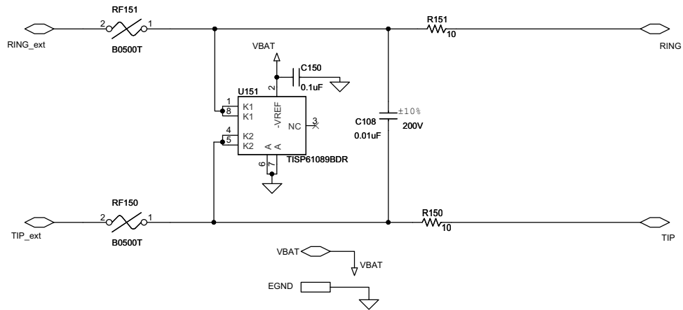
Figure 13. Flyback Protection 1
