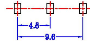
P.C.B LAYOUT BOTTOM VIEW
