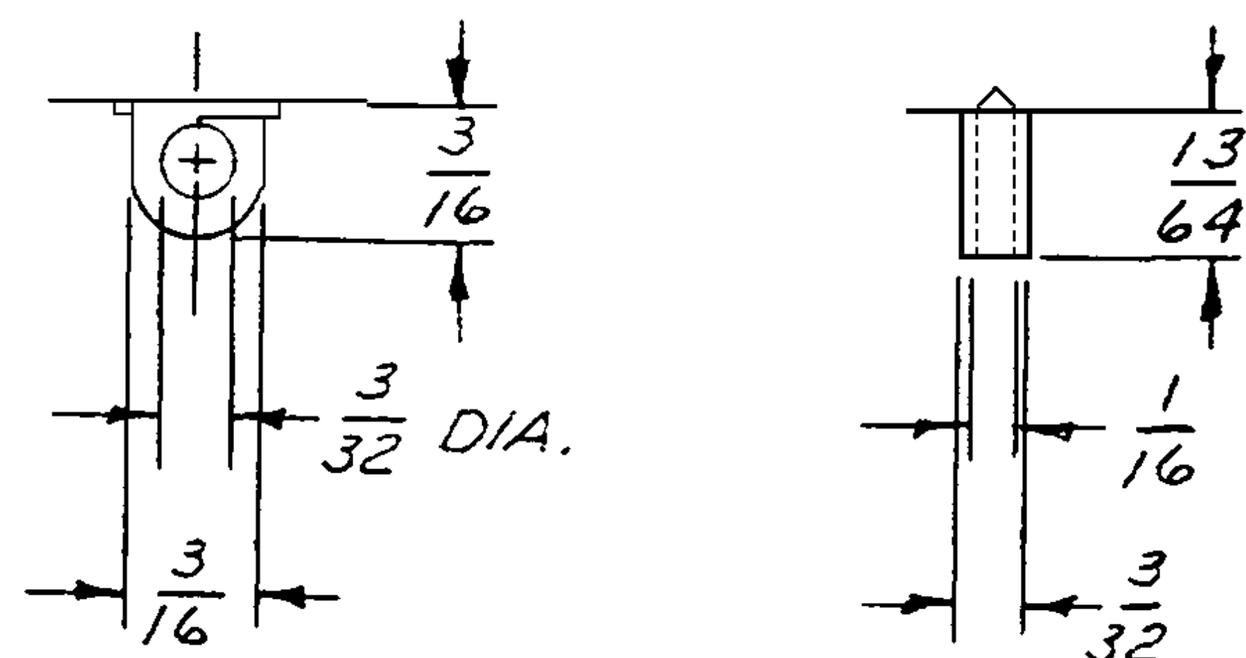
TERMINAL DETAIL
