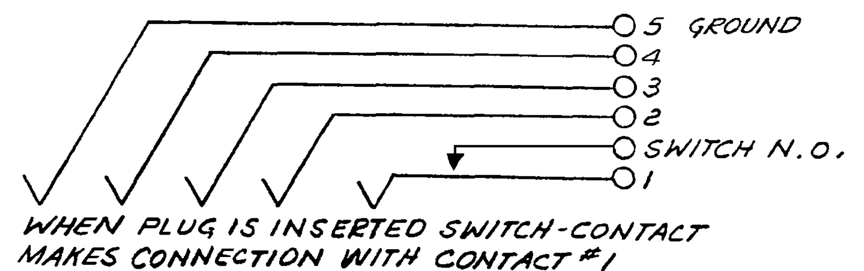
JACK SCHEMATIC
