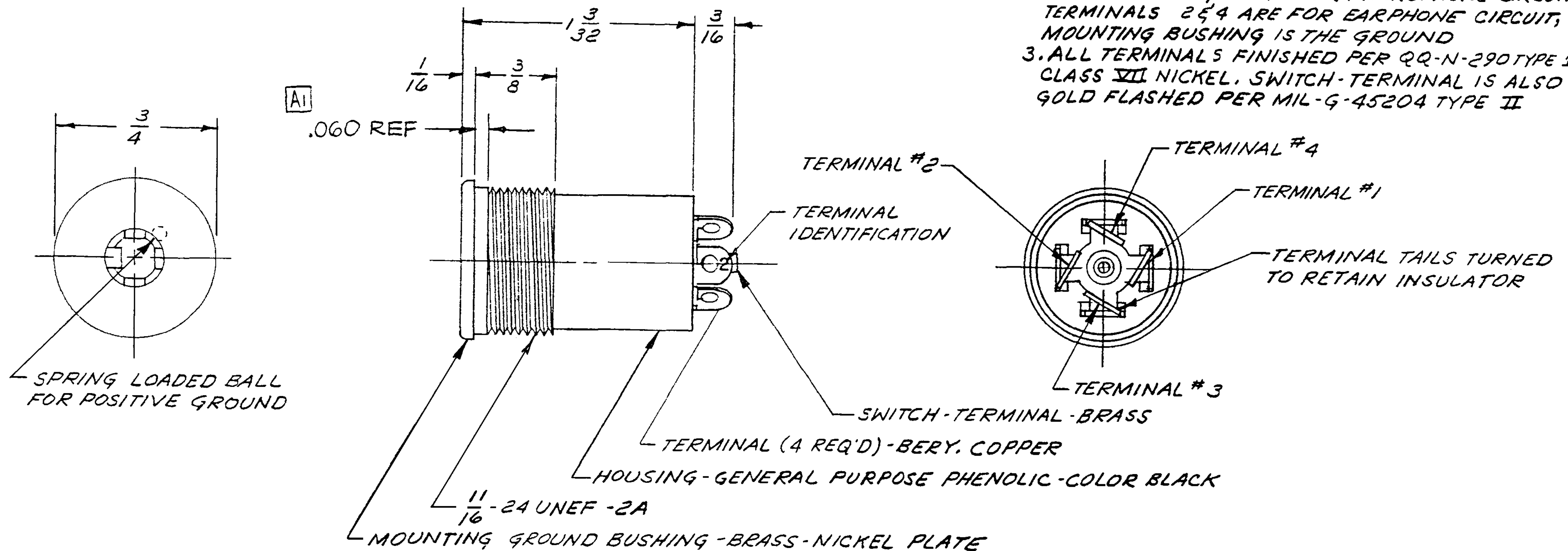
JACK SCHEMATIC
