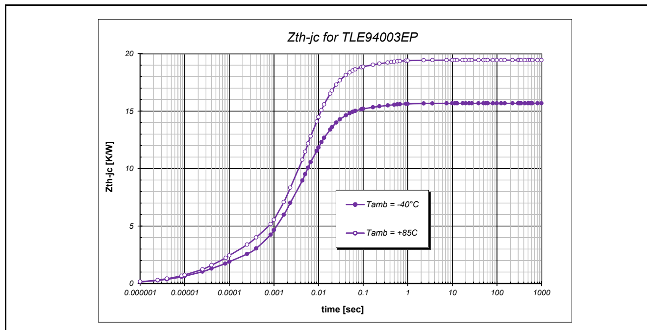
Figure 17 ZthJC Curve
