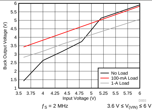
图 1. Buck Output Voltage vs Minimum Input Voltage
