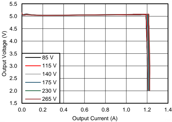
Figure 41. Output V-I Characteristic
