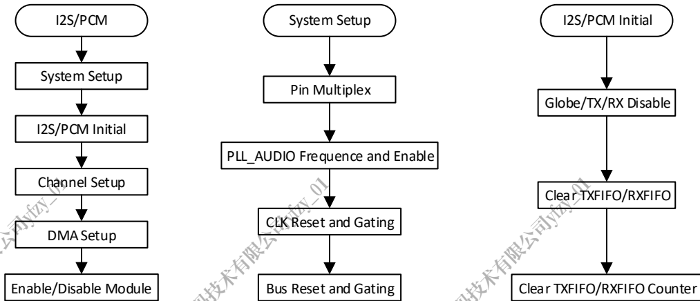
Figure 11-7. I2S/PCM Operation Flow
