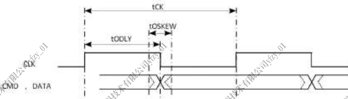
Figure 2-28. SMHC0/1 SDR Mode Output Timing Diagram
