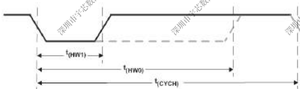
Figure 12-31. Host Bit Timing
