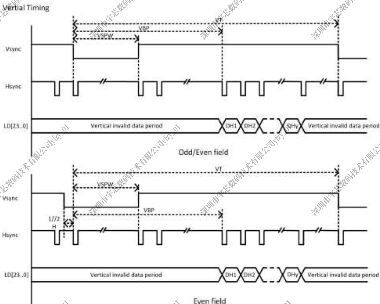
Figure 7-3. HV Interface Vertical Timing
