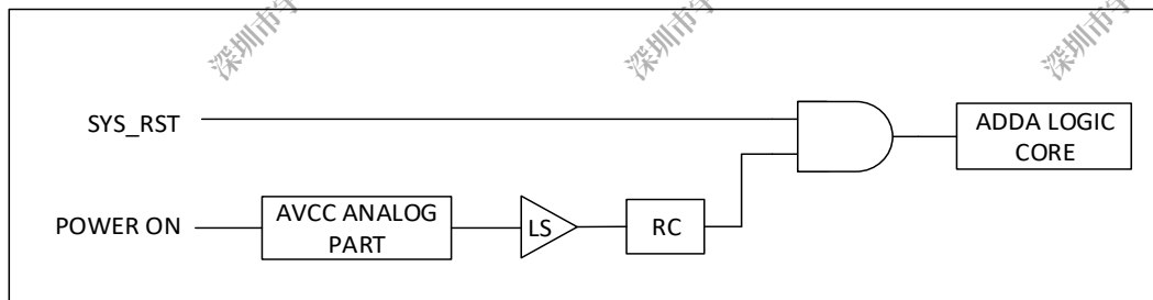
Figure 11-12. Audio Codec Analog Part Reset System
