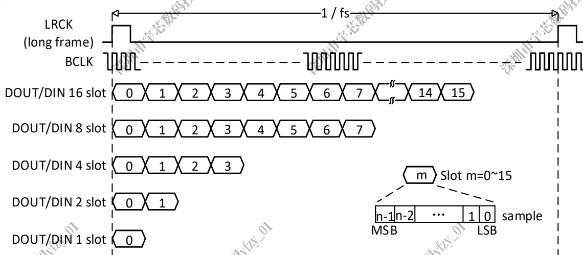
Figure 11-5. PCM Long Frame Mode Timing
