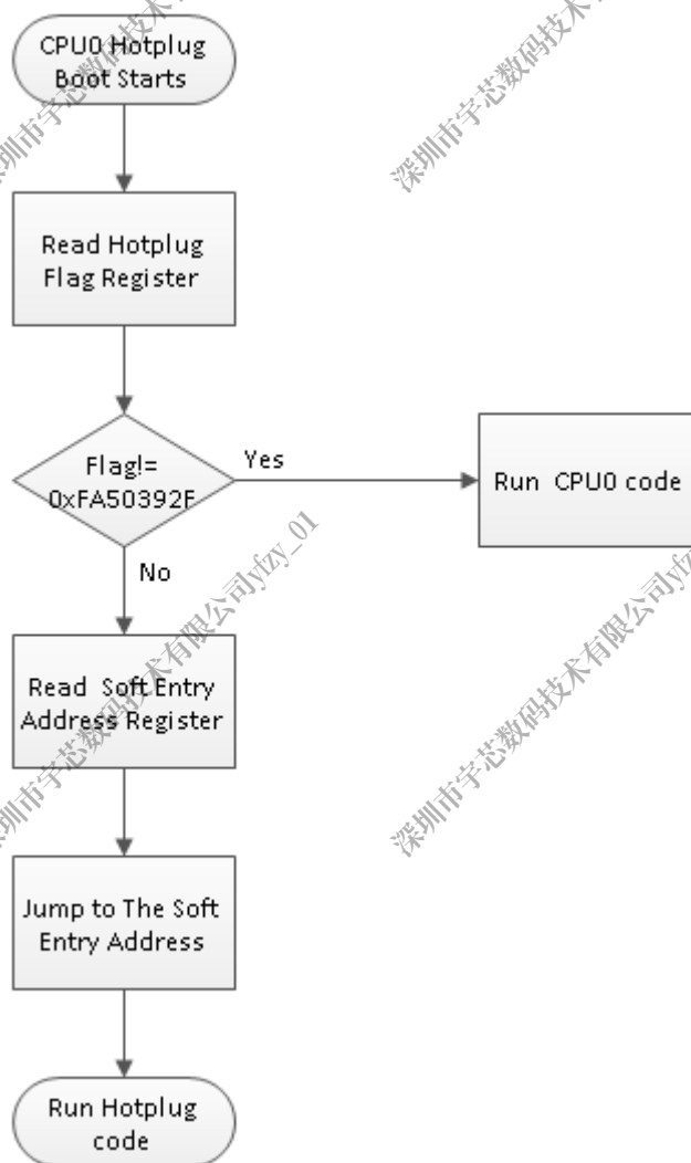
Figure 3-7. CPU0 Hot Plug Process
