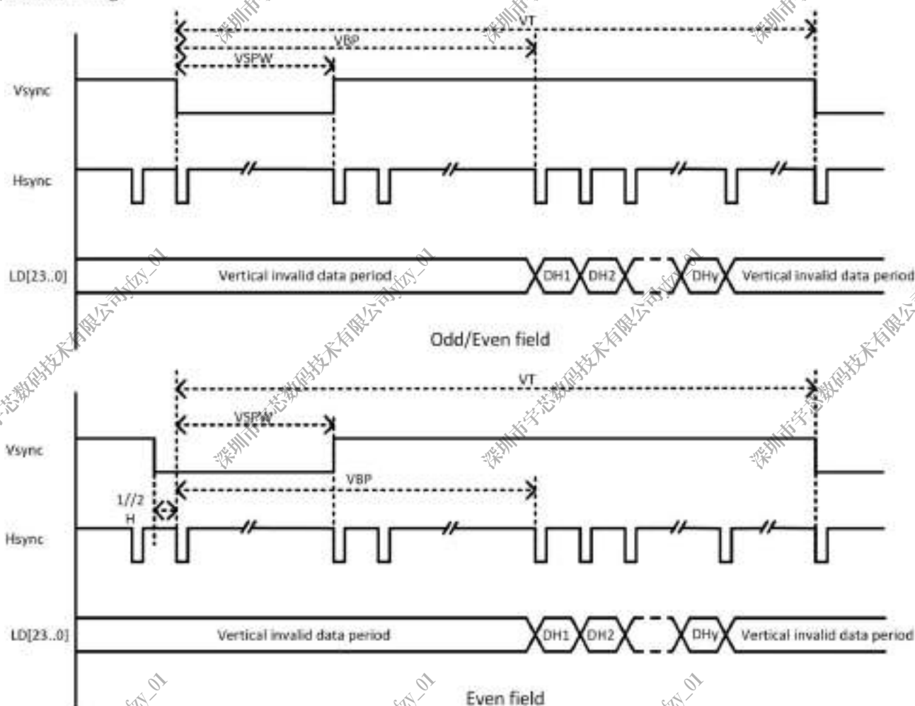
Figure 2-42. HV_IF Interface Vertical Timing
