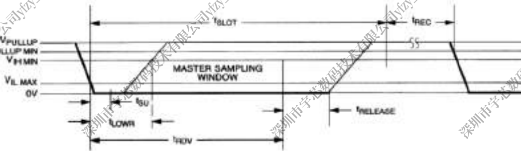
Figure 12-37. Read Data Slot
