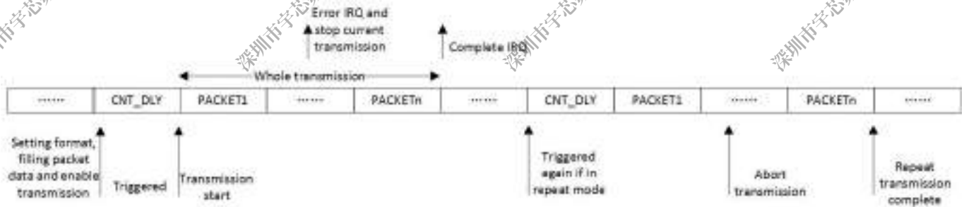
Figure 8-14. CCI Transmission Control
