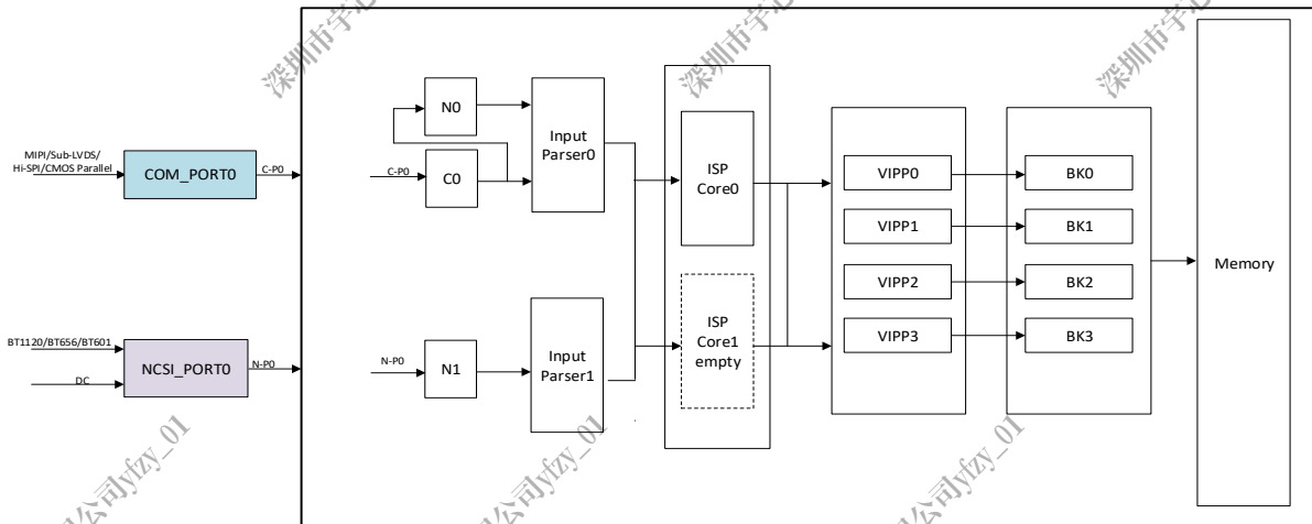
Figure 8-1. CSIC Block Diagram
