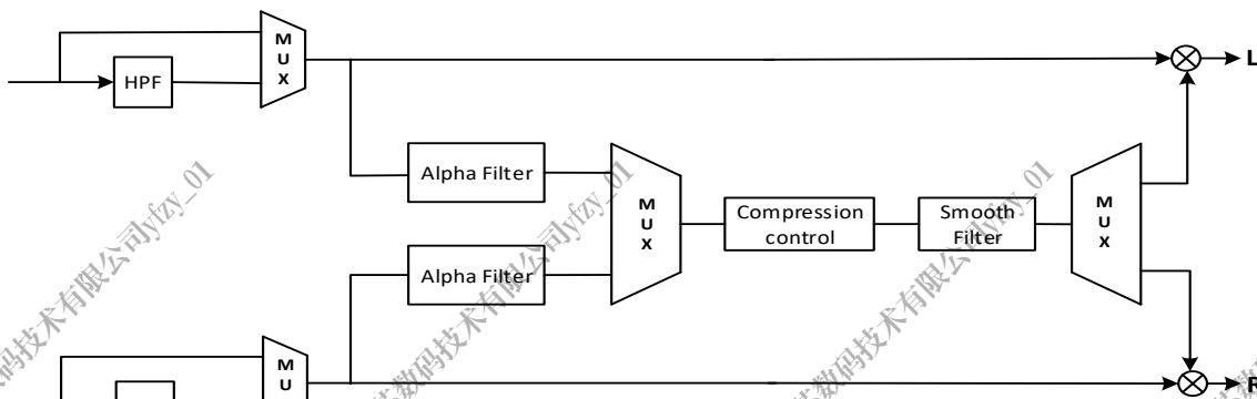
Figure 11-16. DAP Data Flow
