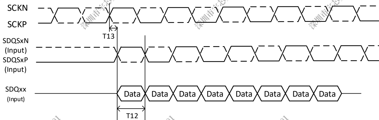
Figure 2-11. DDR3/DDR3L Read Cycle
