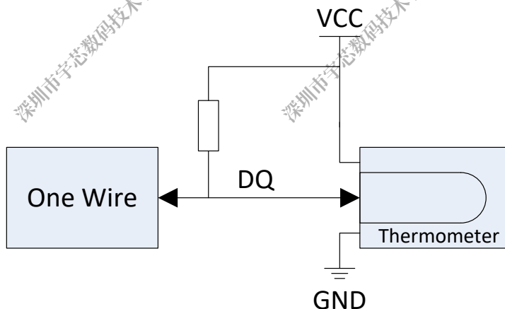
Figure 12-28. Typical Application
