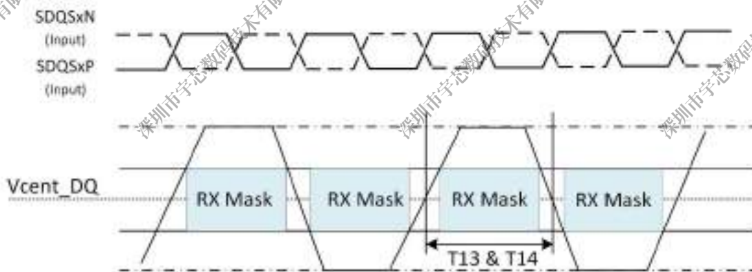
Figure 2-20. LPDDR4 Read Cycle
