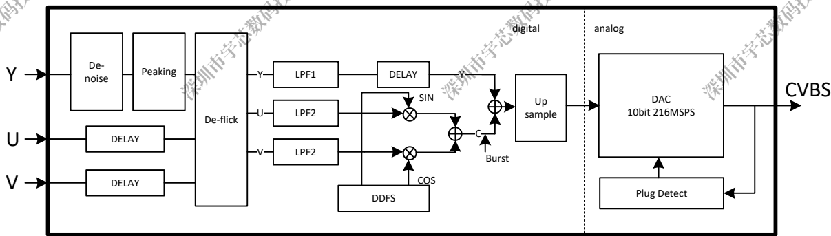
Figure 7-17. TVE Block Diagram
