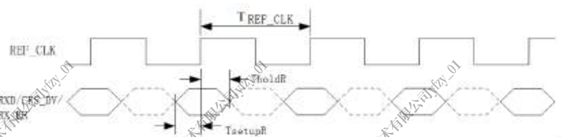
Figure 2-48. RMII Receive Timing
