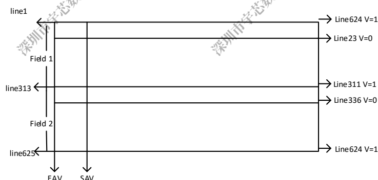
Figure 7-29. BT.656 625line Vertical Timing Diagram
