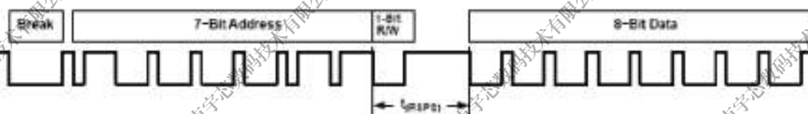
Figure 12-33. t(RSPS) Requirement
