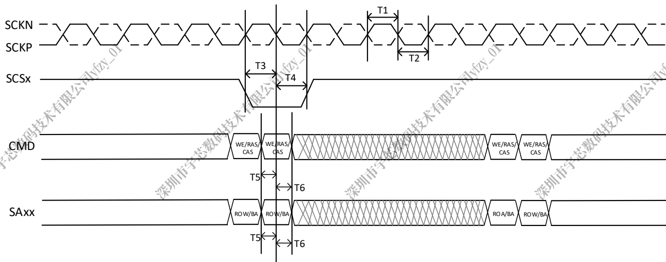
Figure 2-12. LPDDR3 Command and Address Timing Diagram
