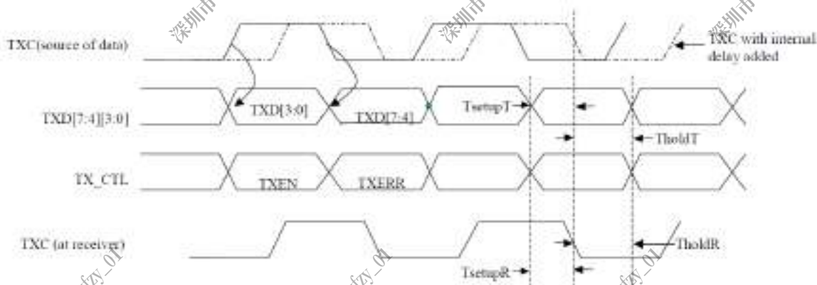
Figure 2-45. RGMII Transmit Timing
