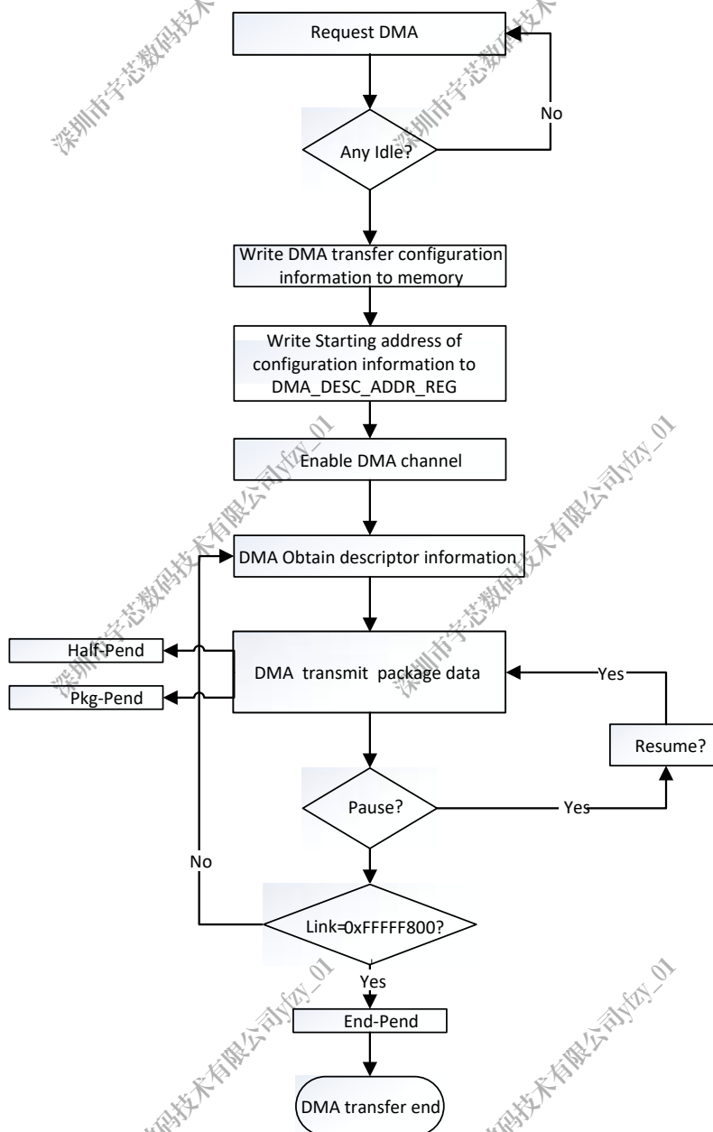
Figure 3-24. DMA Transfer Process
