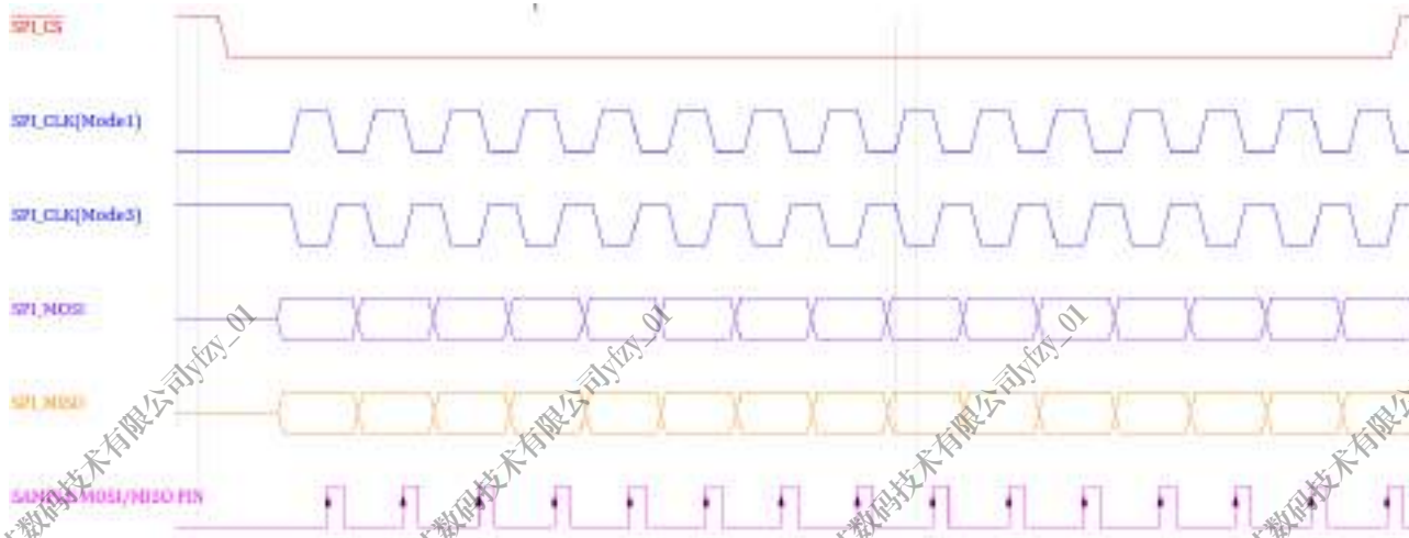
Figure 12-20. SPI Phase 1 Timing Diagram
