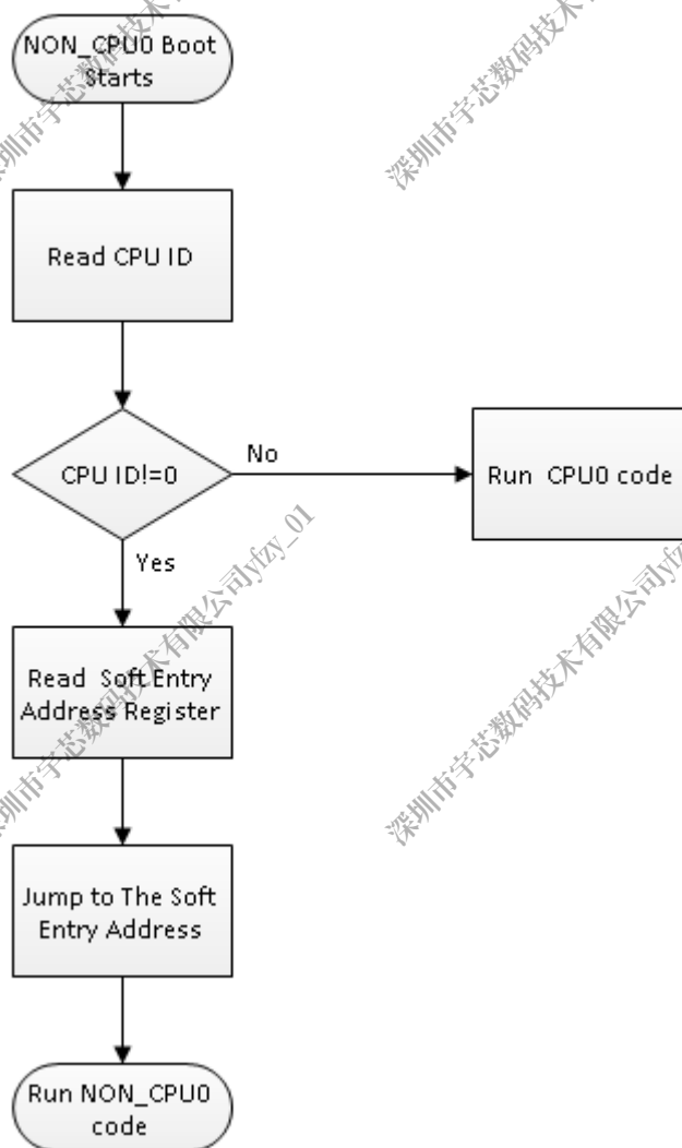
Figure 3-6. NON_CPU0 Boot Process
