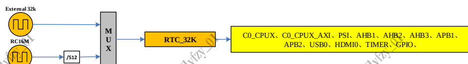
Figure 3-4. Module Clock Tree
