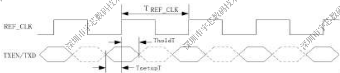
Figure 2-47. RMII Transmit Timing
