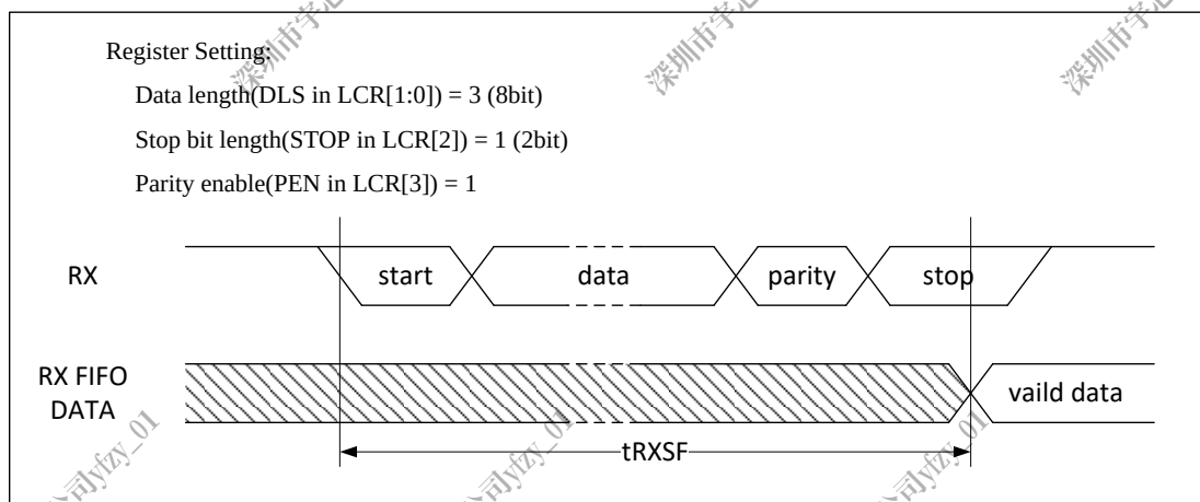
Figure 2-54. UART RX Timing
