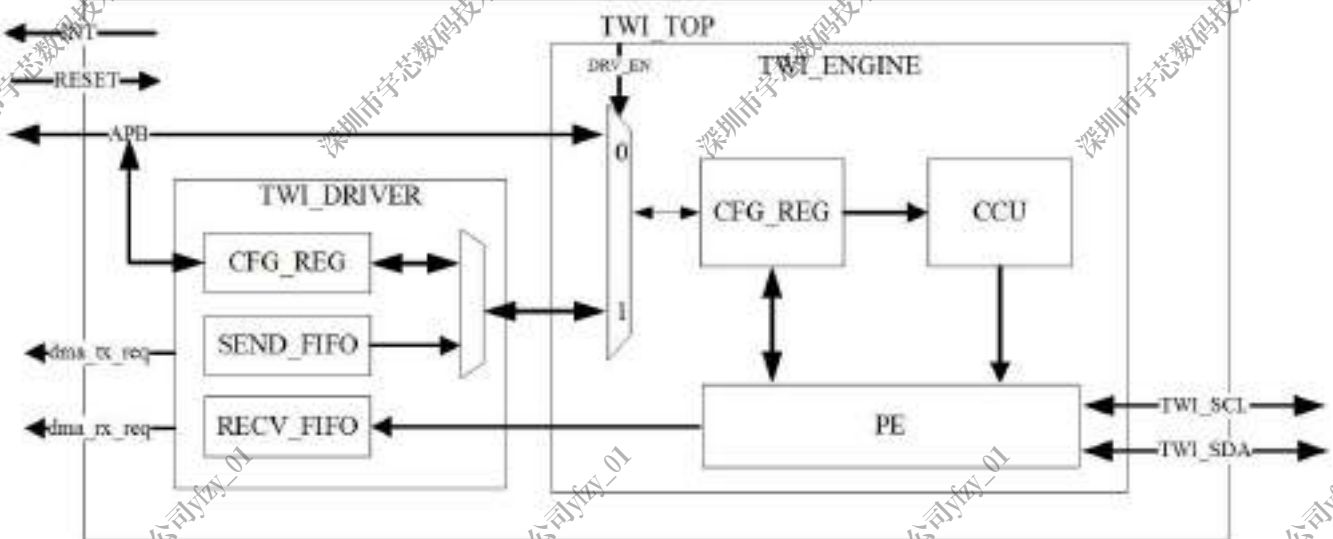
Figure 12-1. TWI Block Diagram
