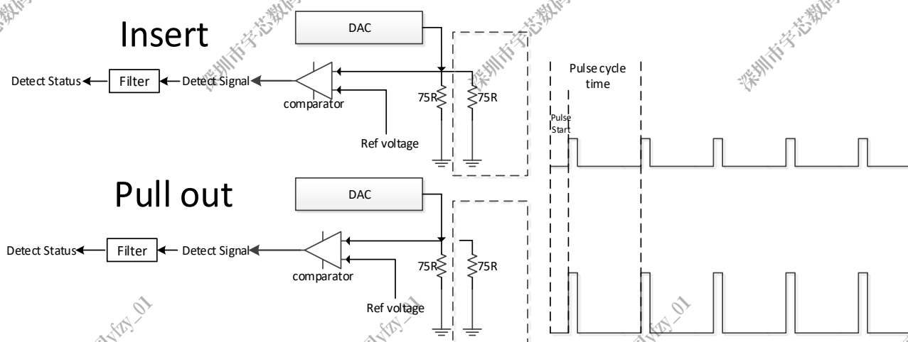
Figure 7-19. Auto Detect Function
