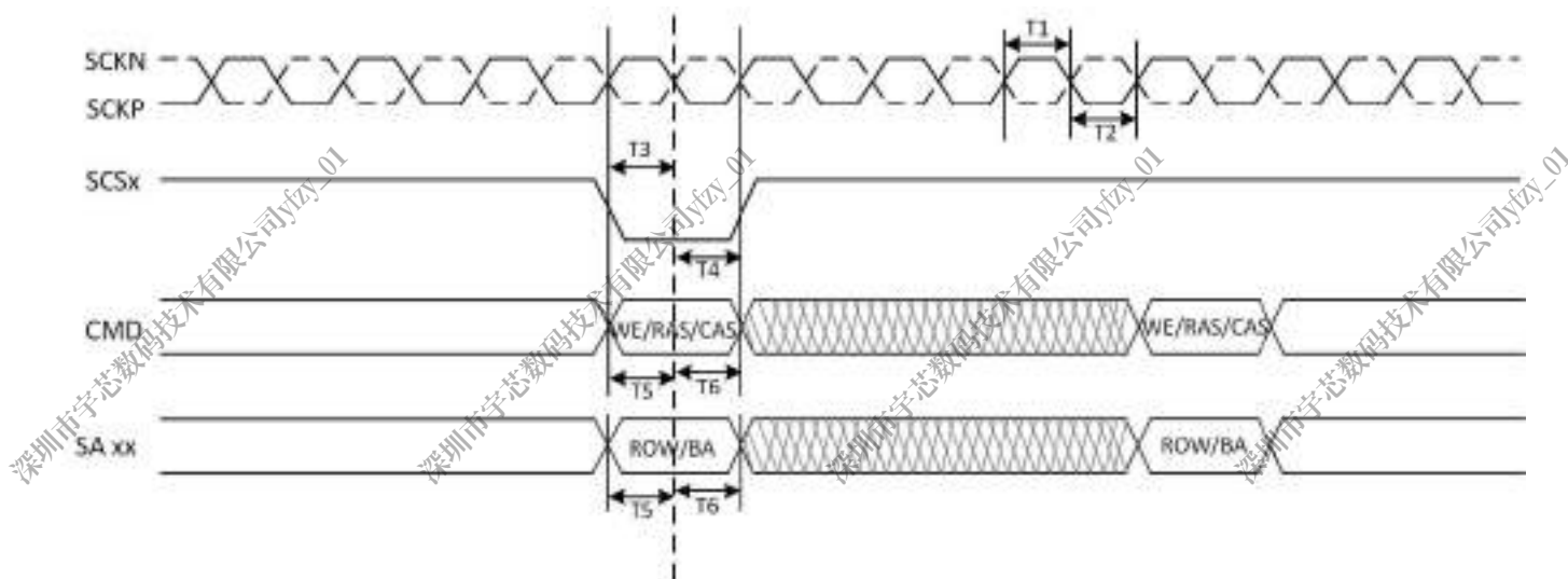
Figure 2-15. DDR4 Comman and Address Timing
