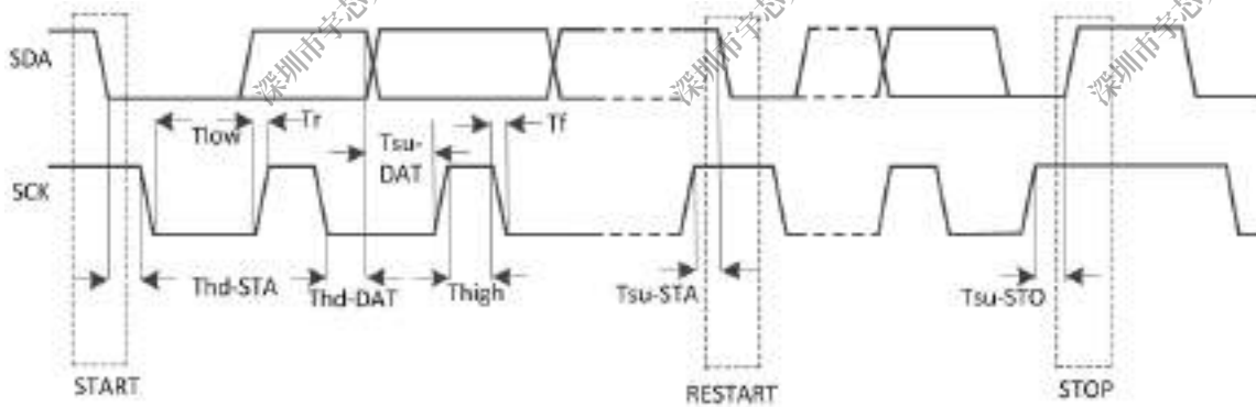
Figure 2-57. TWI Timing
