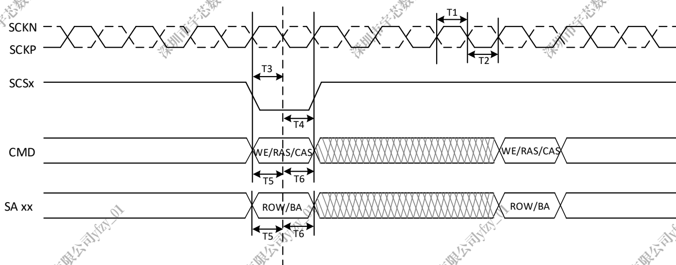
Figure 2-9. DDR3/DDR3L Command and Address Timing
