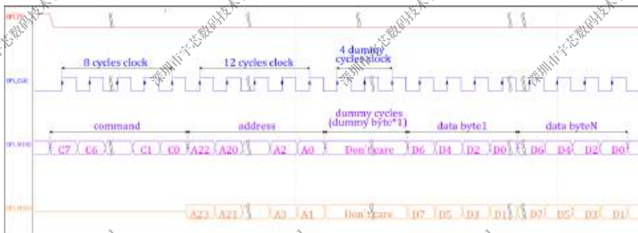
Figure 12-23. SPI Dual IO Mode
