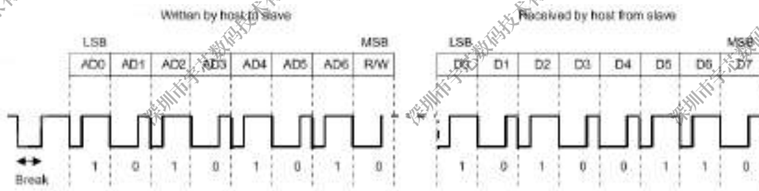
Figure 12-29. Typical Read Cycle
