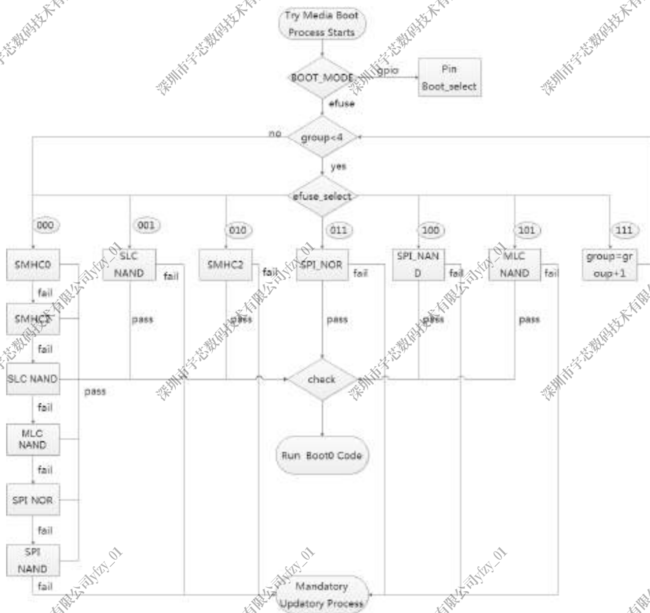
Figure 3-14. eFuse Boot Select Process
