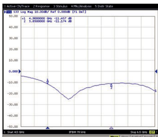
Antenna S11 on Test Board
