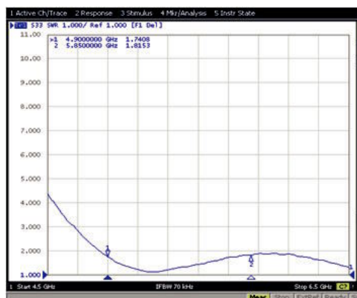
Antenna VSWR on Test Board
