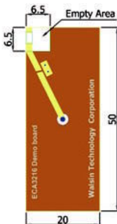
Empty Space 6.5 mm x 6.5 mm
