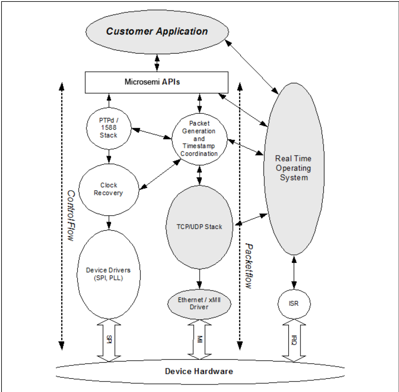
Figure 37 - High Level Software Architecture
